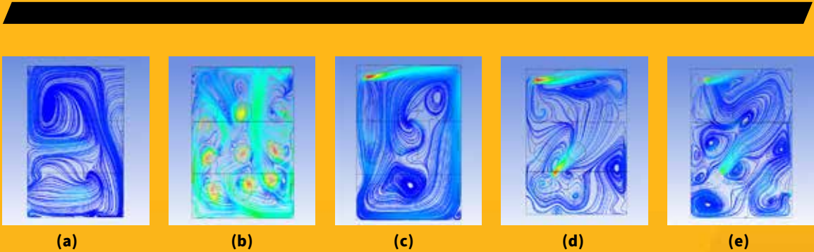
Velocity streamline contours for (a) baseline case simulation, (b) simulation with ceiling fans and an exhaust fan switched on, (c) simulation with one exhaust fan and one pedestal fan, (d) simulation with one exhaust fan and two pedestal fans, and (e) simulation with two exhaust fans and two pedestal fans
