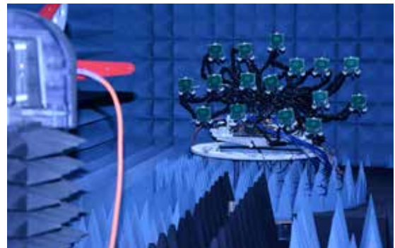
The MEDUSA platform
